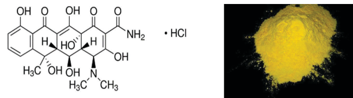
Figure 2. Chemical structure of oxytetracycline-hydrochloride (left) and physical appearance (right).
